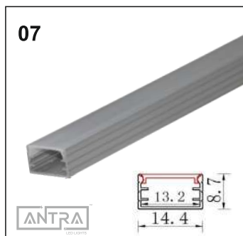
14mm SURFACE
