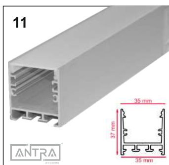
35mm SURFACE
