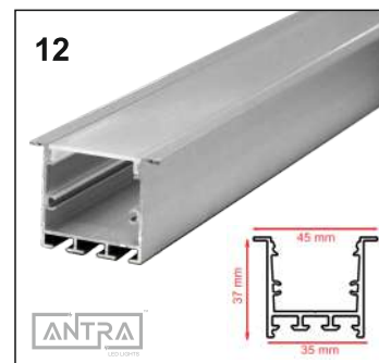
35mm CONCEALED
