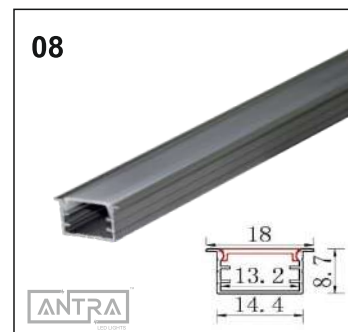
14mm CONCEALED
