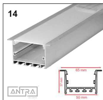
50mm CONCEALED
