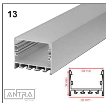
50mm SURFACE
